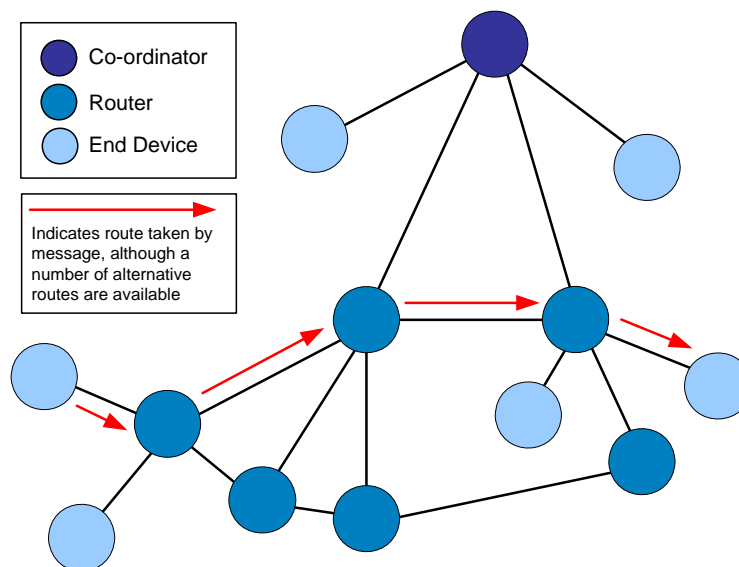
Figure 7: Mesh Topology
