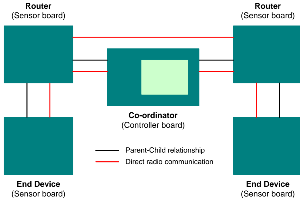
Figure 10: Example Demo System Topology
