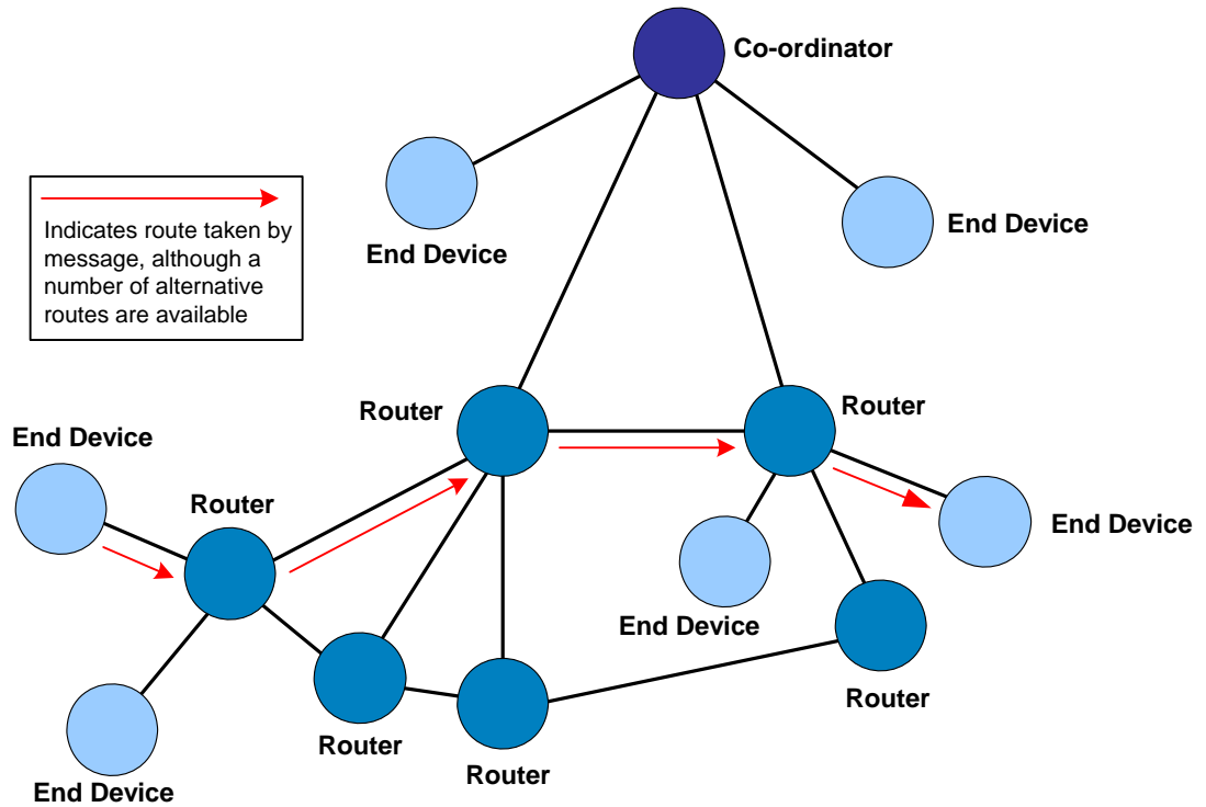
Figure 5: Mesh Topology
