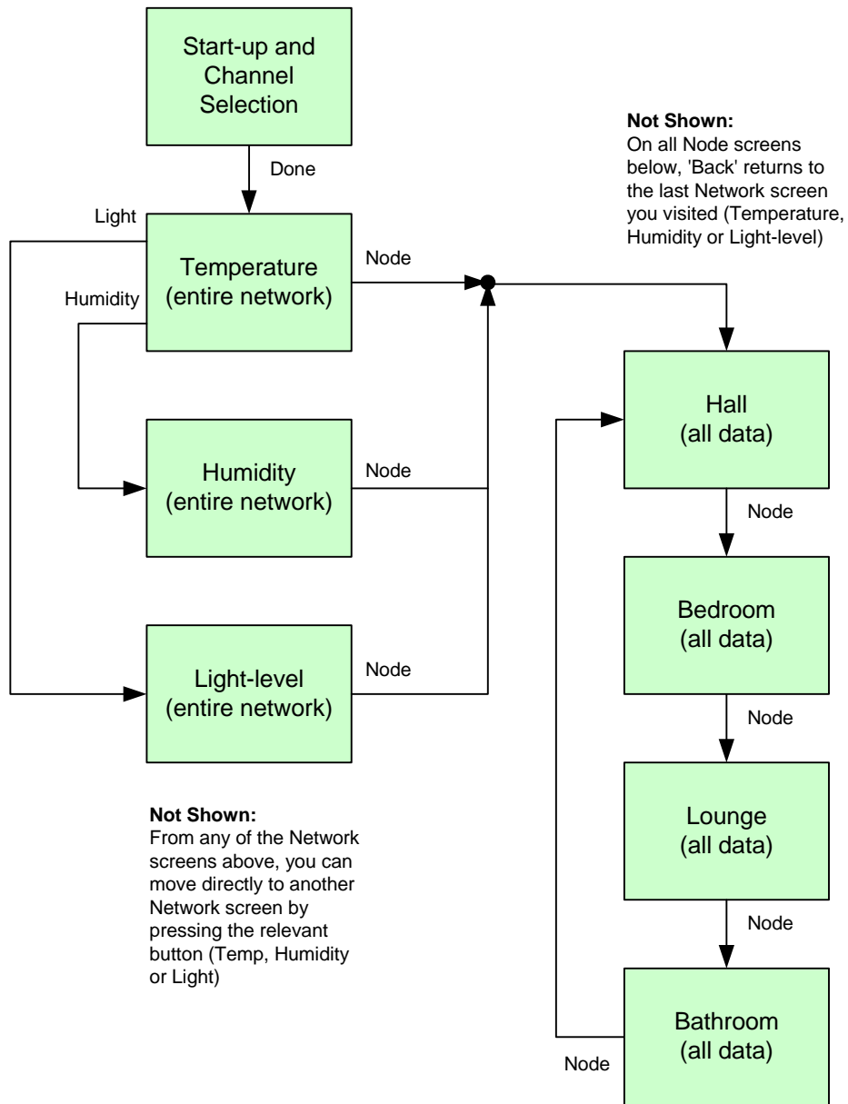
Figure 9: Screen Navigation on Controller Board
